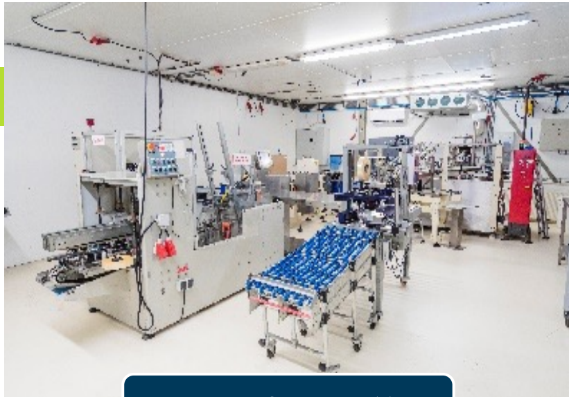
Horizontal cartoning (2)
